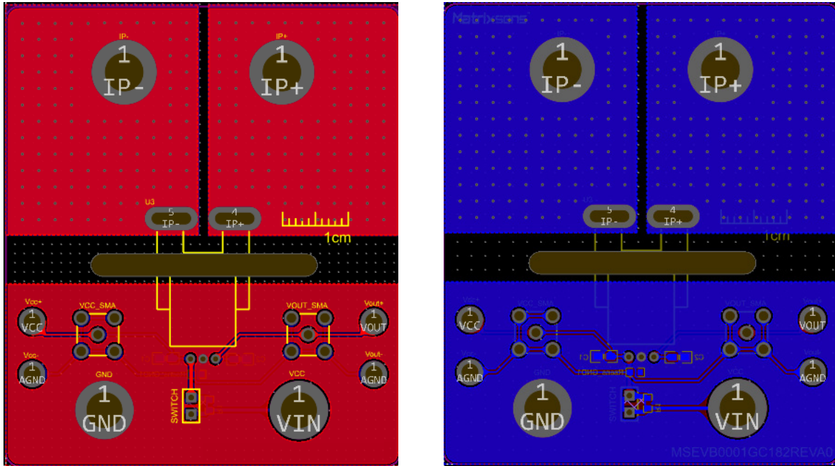
Figure 13. Demo board
