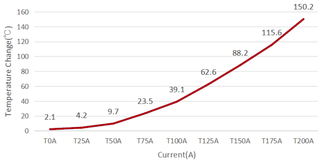
Figure 7. Thermal curve
