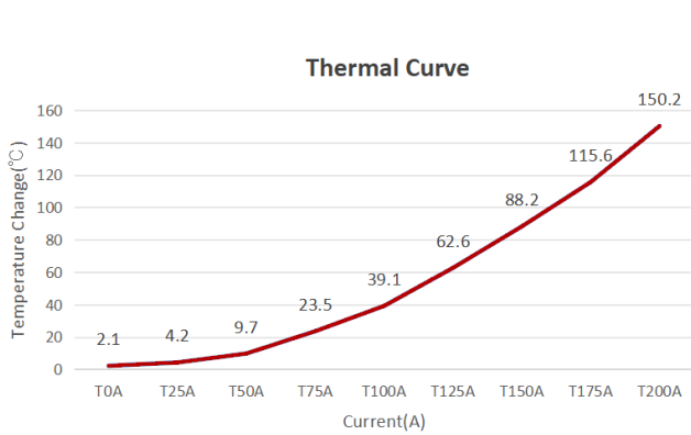
Figure 7. Thermal curve
